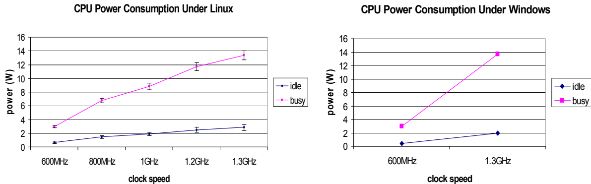
Figure 2: CPU power consumption under Linux and Windows
