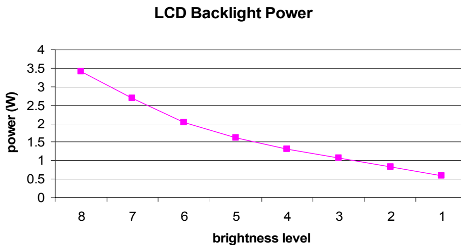
Figure 1: Backlight power versus brightness level
