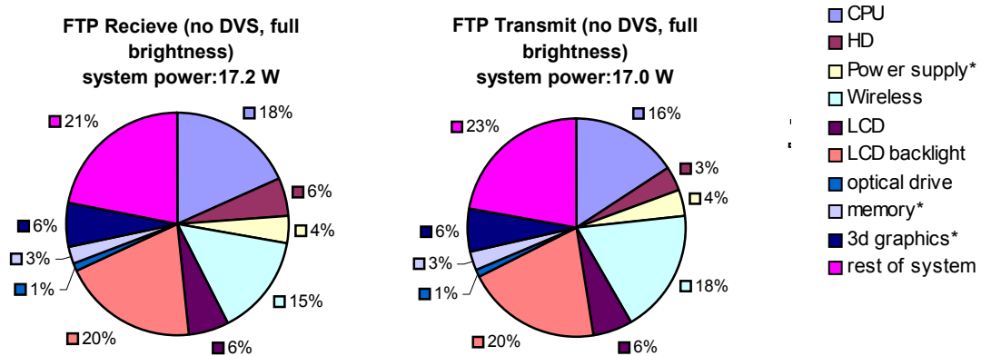
Figure 6: Power consumption breakdown of FTP
