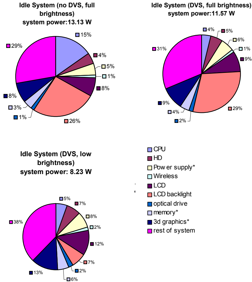
Figure 4: Breakdown of idle system power conversion with various CPU speeds and display brightness levels
