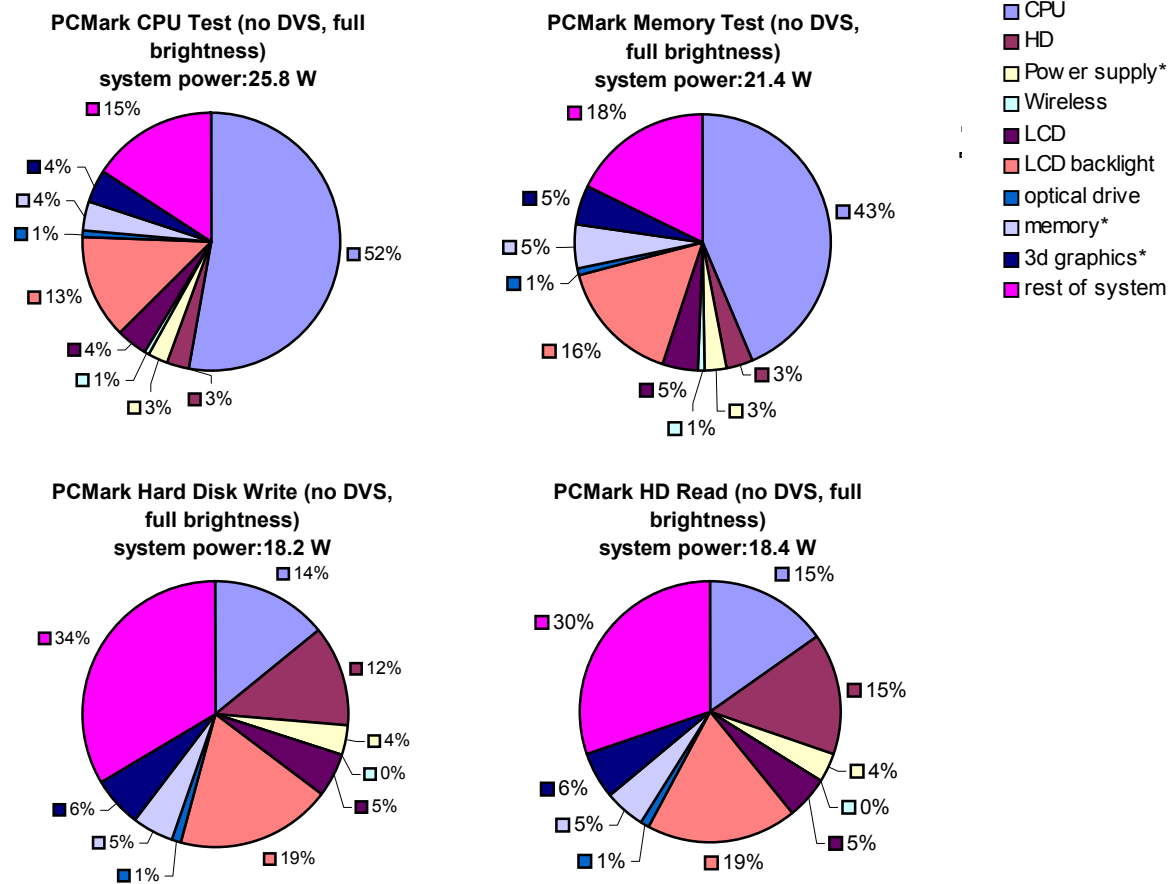
Figure 5: Breakdown of power consumption under different PCMark2002 benchmarks
