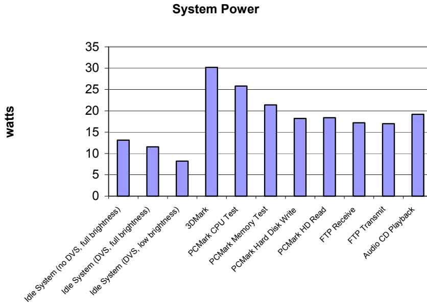
Figure 3: Power consumption of system under various workloads
