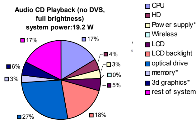
Figure 7: Power consumption breakdown of audio CD playback
