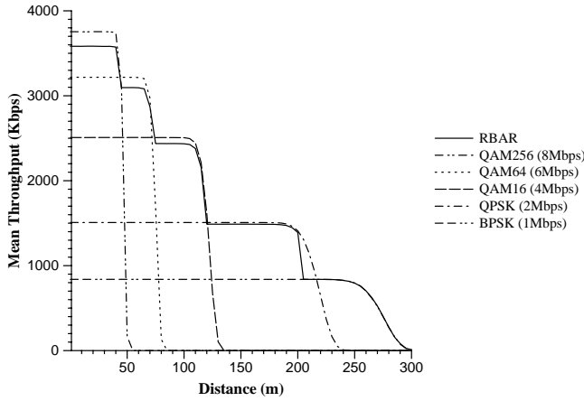
Figure 12: Performance of RBAR for a single CBR connection between two nodes at fixed distances.
