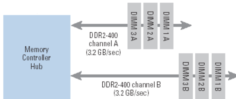
Figure 1: A maximally loaded memory subsystem.
